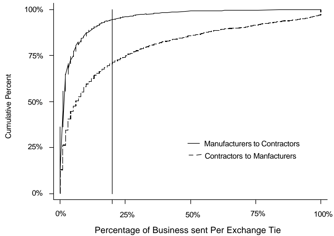
Figure 1: Cumulative Distribution of All Exchange Ties
