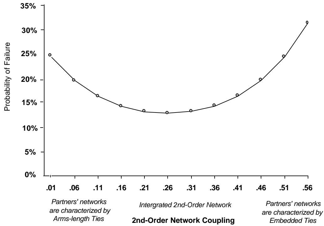
Figure 4: Predicted Effect of 2nd-Order Network Coupling on Failure
