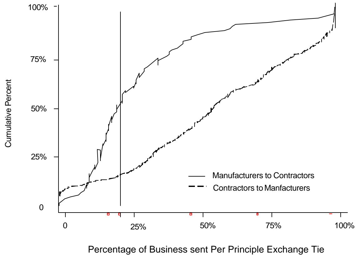
Figure 2: Cumulative Distribution of Principle Exchange Ties
